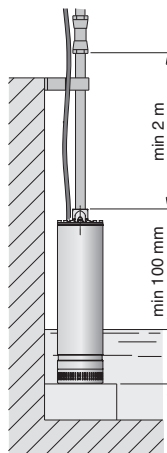
3.93.007/2 Construction without float switch
