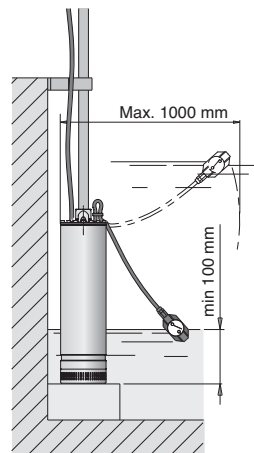
3.93.007/3 Construction with float switch
