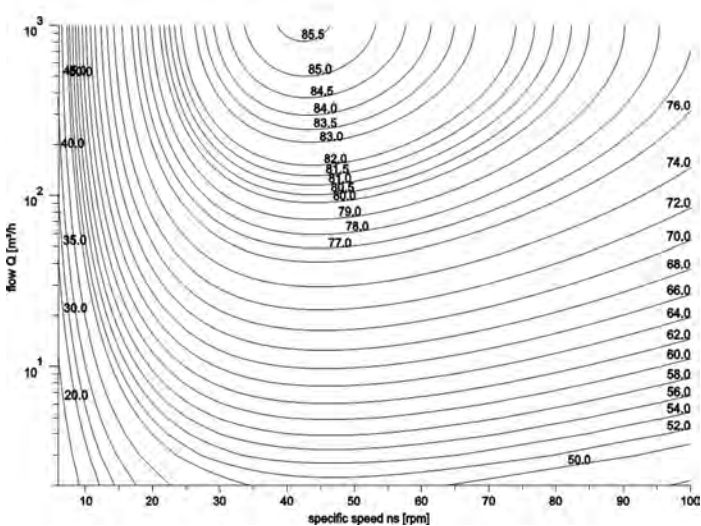
MEI = 0.7 for ESCC 2900rpm
