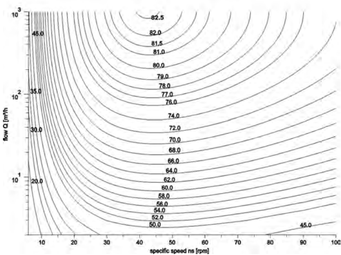
MEI = 0.4 for ESCC 2900 rpm
